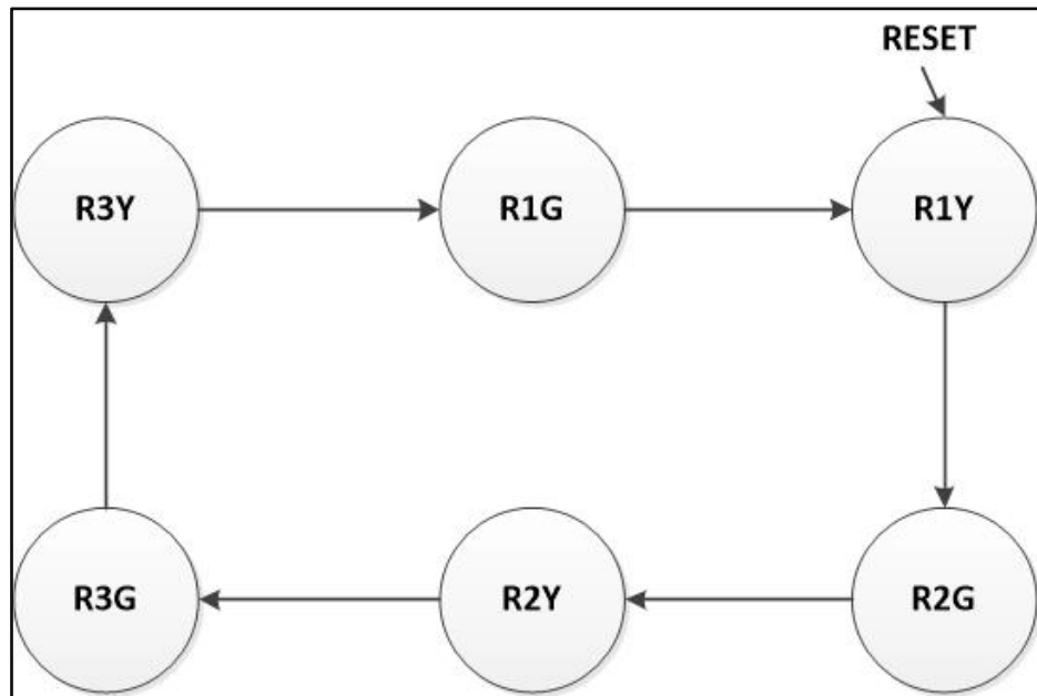
Fig. 3. The normal flow of the system's states.
