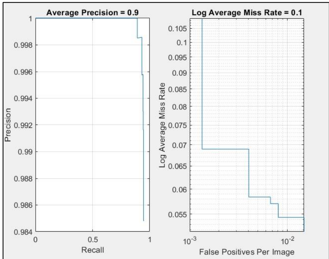
Fig. 23. Evaluation of license plate detector.
