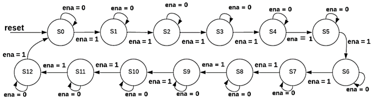
Figure (4.12) Finite State Machine FSM diagram.
