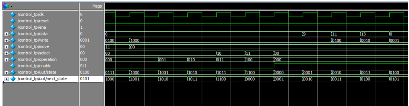
Figure (4.21) Simulation of control "select register and executed the operation".
