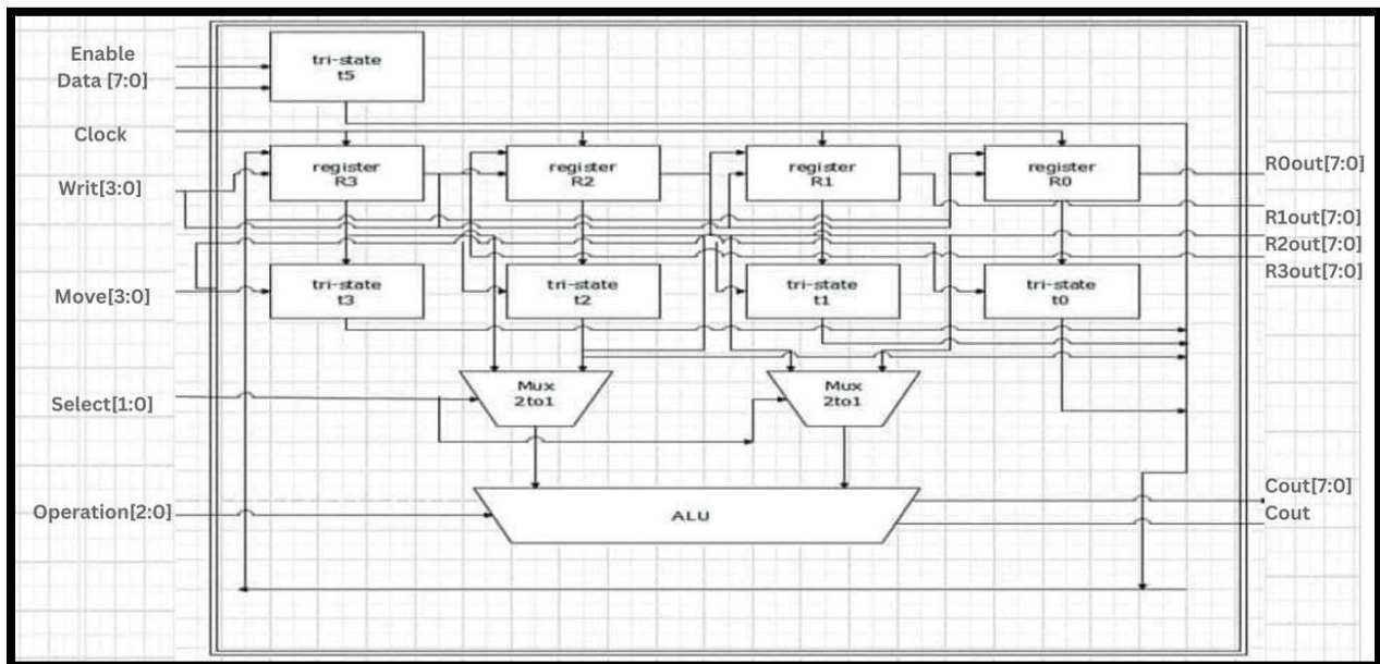
Figure (4.5) Tri-state top-level schematic.
