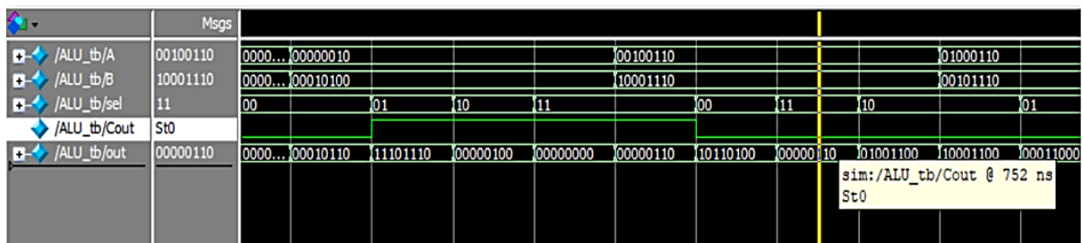
Figure (4.13) ALU operation.
