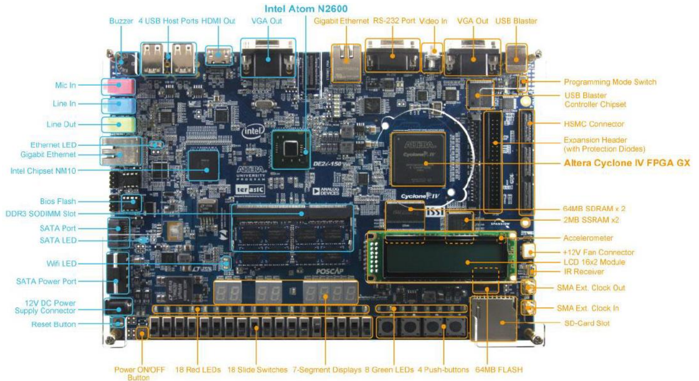
Figure (2.2) Altera Cyclone IV GX FPGA development board.
