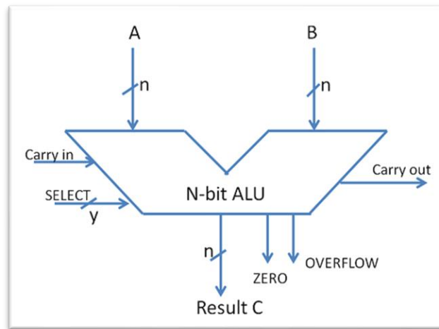
Figure (4.3) Arithmetic Logic Unit.
