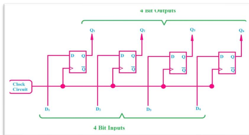
Figure (4.1) D flip-flops.
