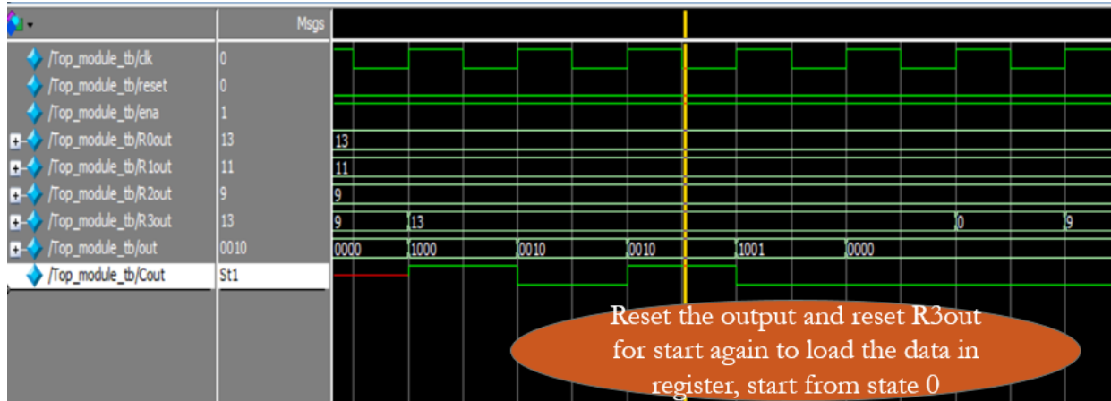
Figure (4.23) Simulation of the top module show executed the operations ADD, SUB, SHL, AND.
