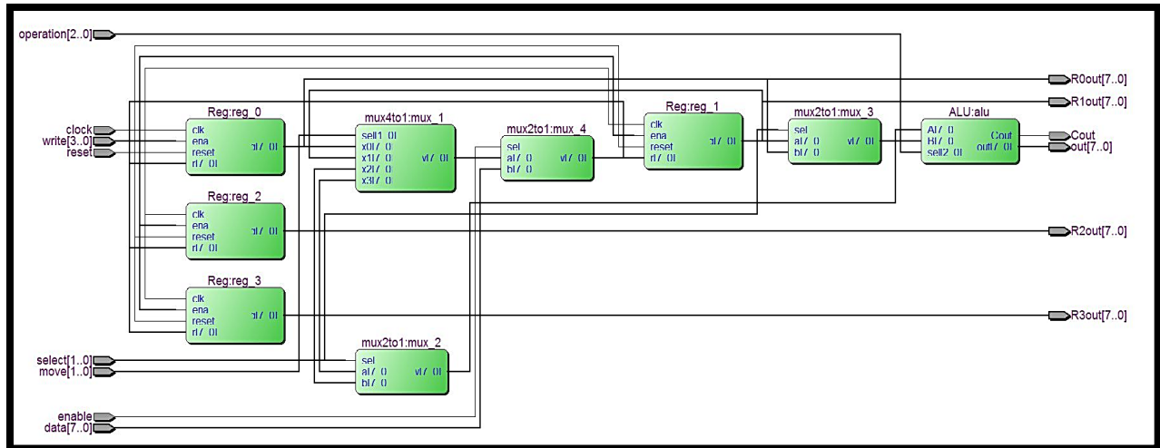
Figure (4.25) Register transfer level schematic for data path MUX 8_bit.
