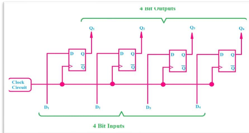
Figure (4.6). D flip-flops.
