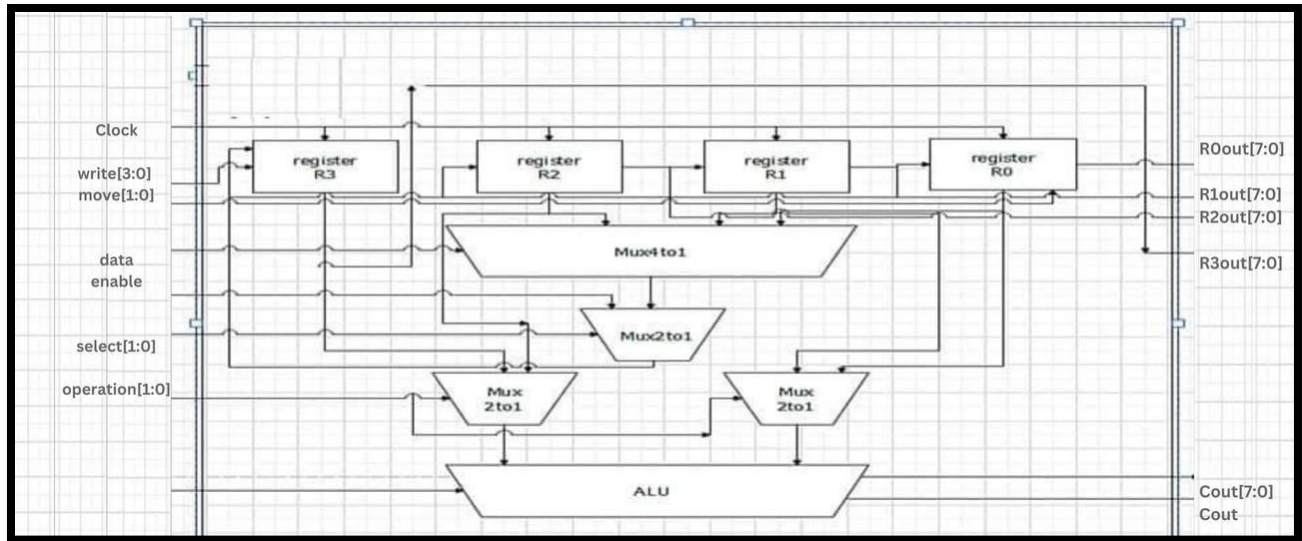
Figure (4.10) MUX top-level schematic.
