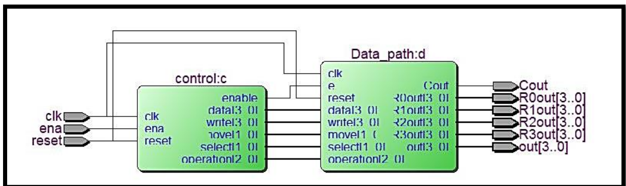
Figure (4.28) Register transfer level schematic for top module MUX.
