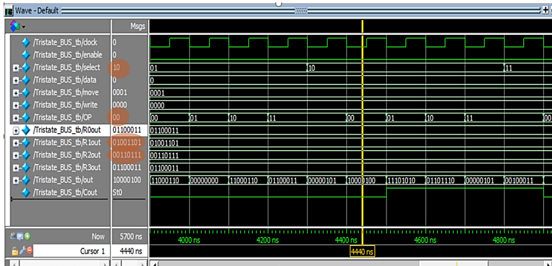
Figure (4.16) ALU "ADD" operation.
