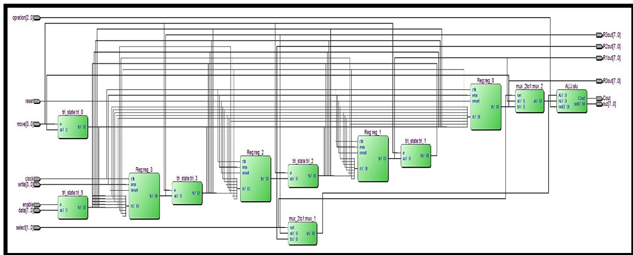
Figure (4.24) Register transfer level schematic for data path Tristate 8_bit.
