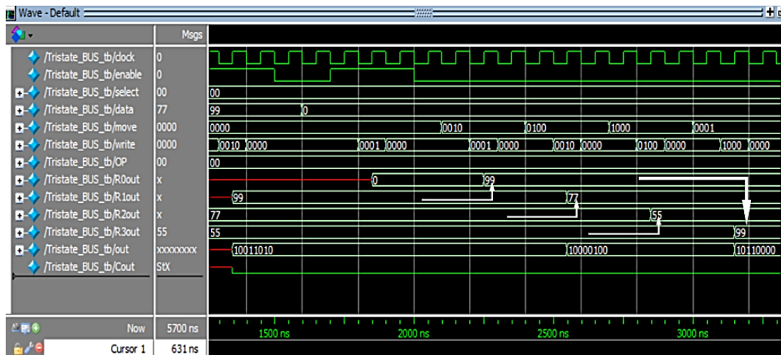
Figure (4.15) The transfer via bus to different registers.
