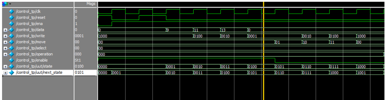
Figure (4.20) Simulation of control "enter data in registers and shifting between registers".
