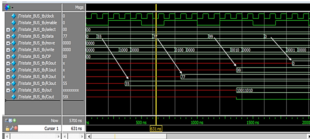
Figure (4.14) Simulation of the tri-state.
