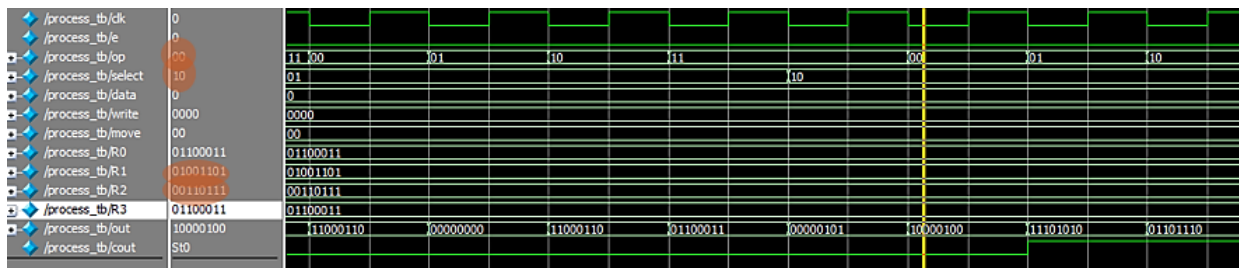
Figure (4.19) ALU "ADD" operation.
