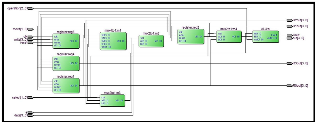
Figure (4.26) Register transfer level schematic for data path MUX 4-bit.
