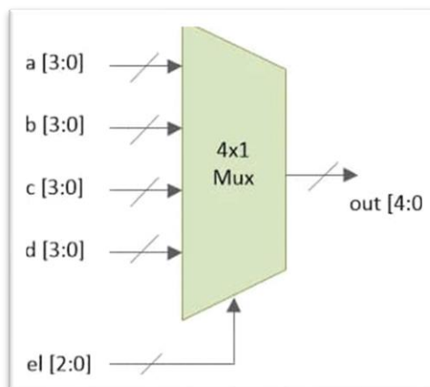
Figure (4.9) Arithmetic Logic Unit.
