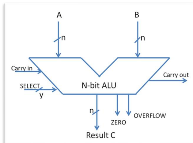
Figure (4.7) Arithmetic Logic Unit.
