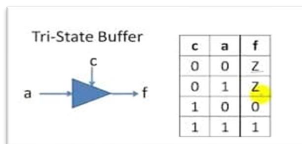
Figure (4.2) Tri-state buffers.
