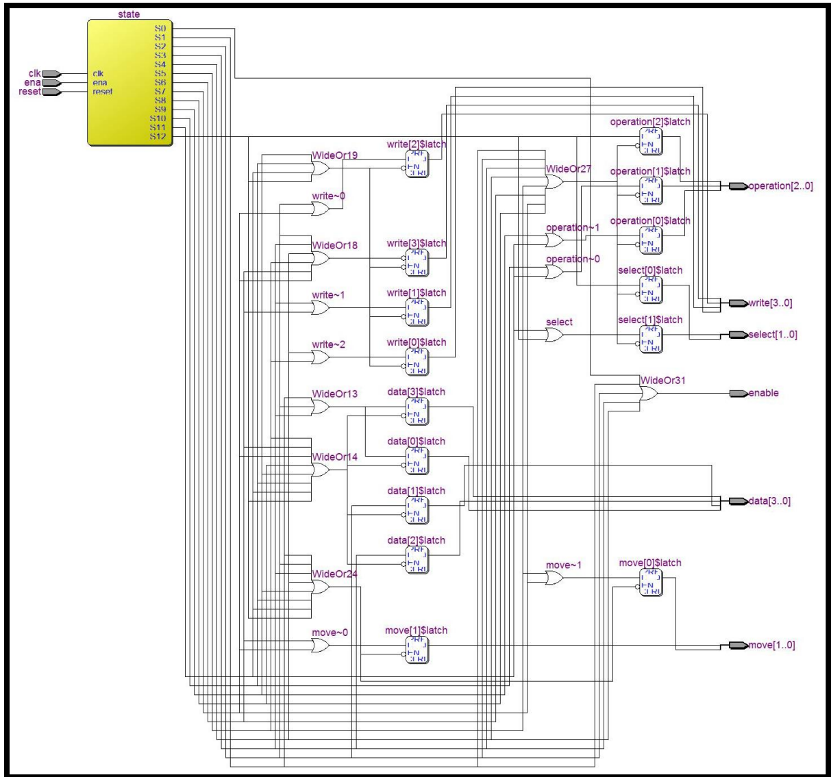
Figure (4.27) Register transfer level schematic for control MUX.
