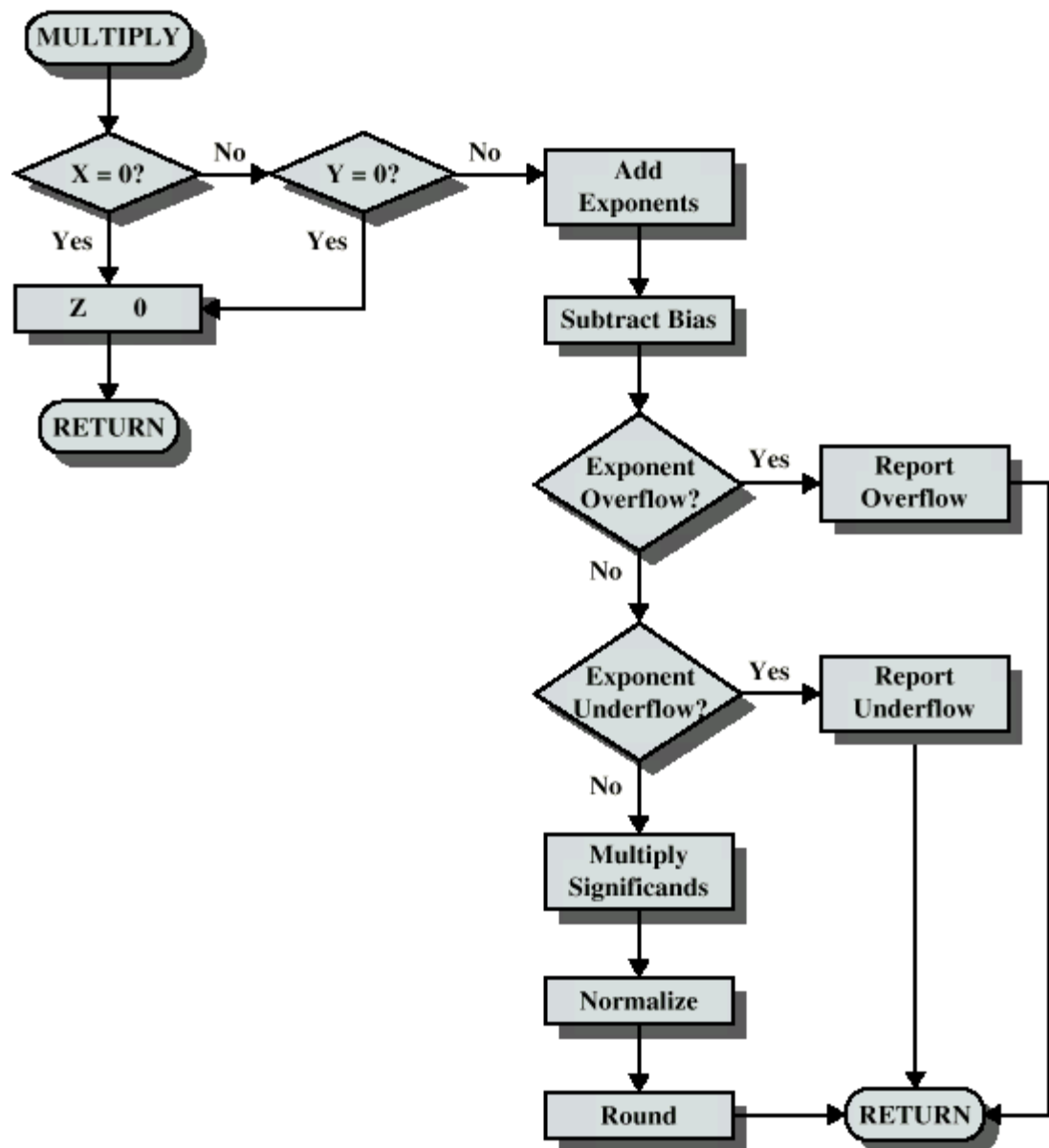
Figure 13: Floating Point Multiplication Flowchart
